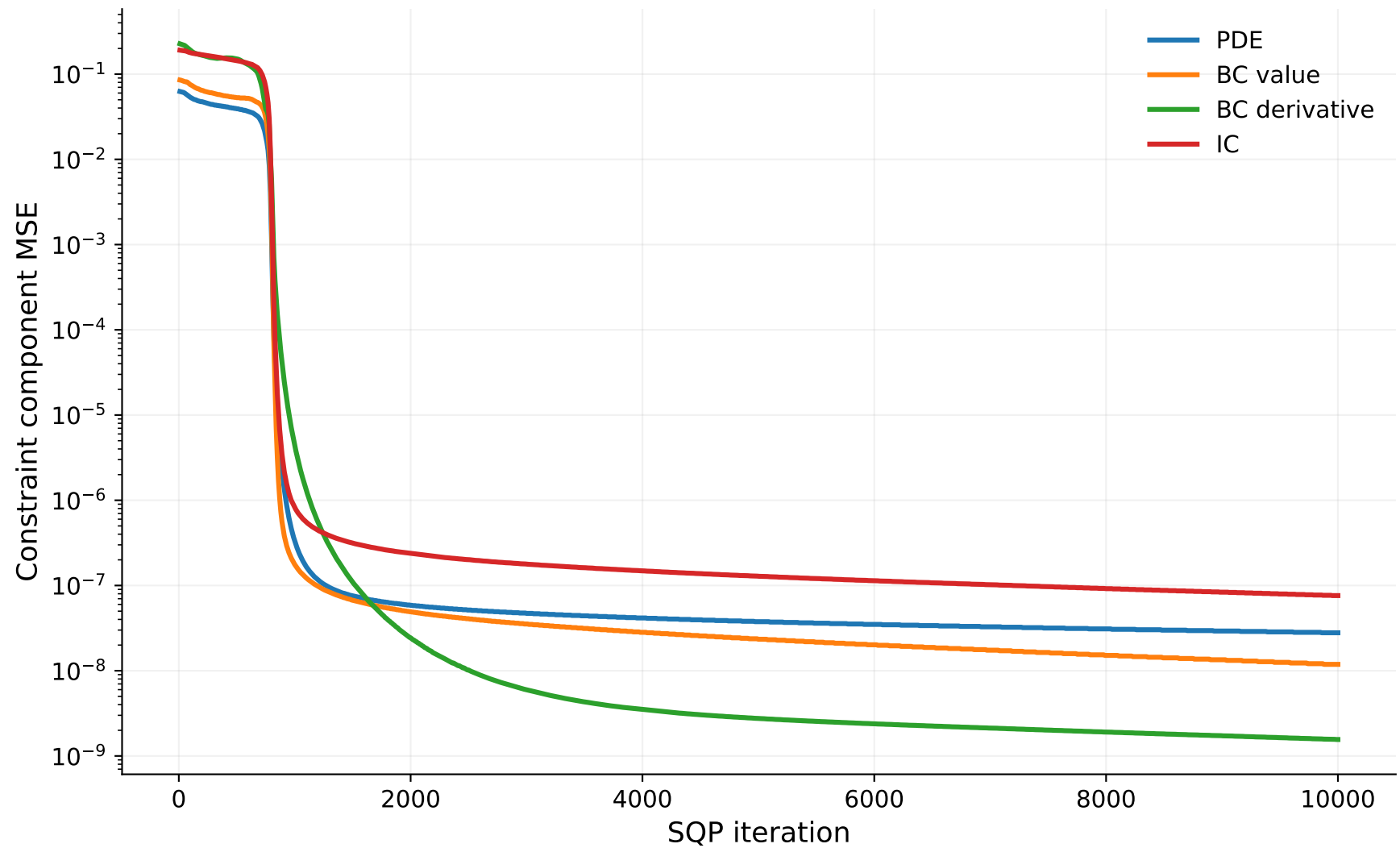
Allen-Cahn equation: deterministic SQP constraint components
